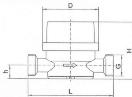
Picture No.4 Installation dimensions
